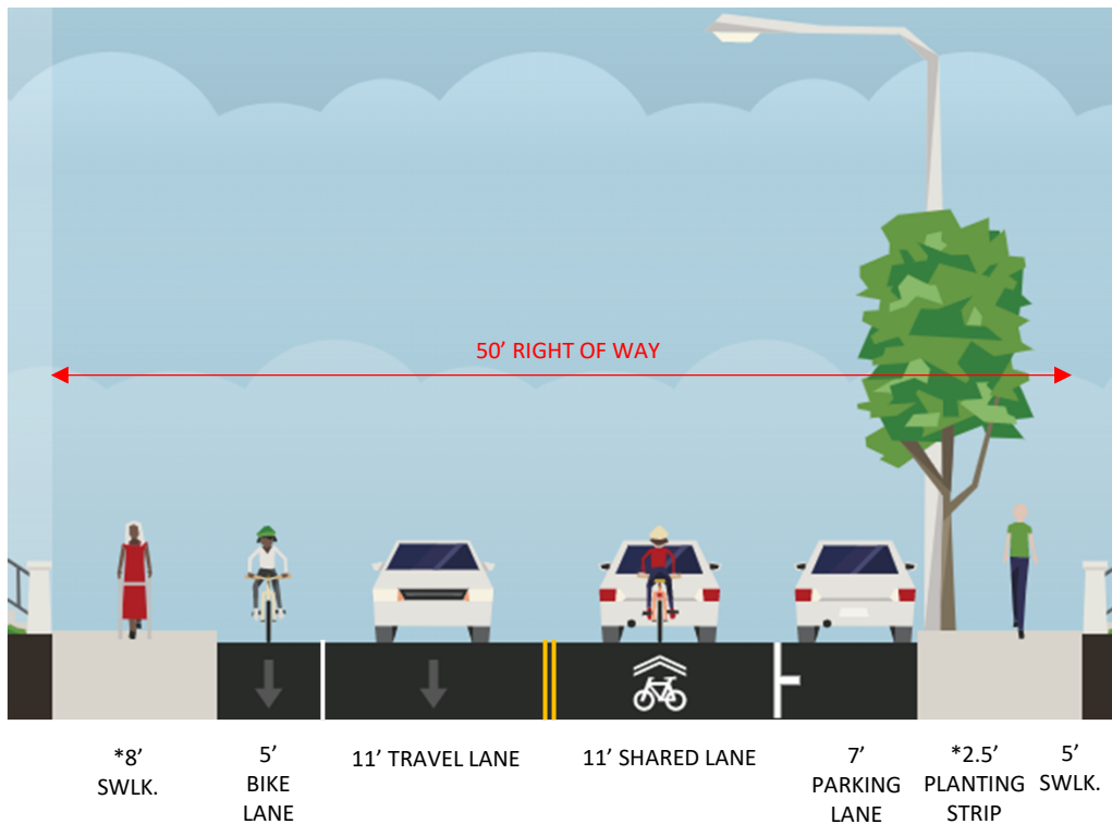
Proposed Layout – Option 1 – Shared Lanes – No Bicycle Accommodations
