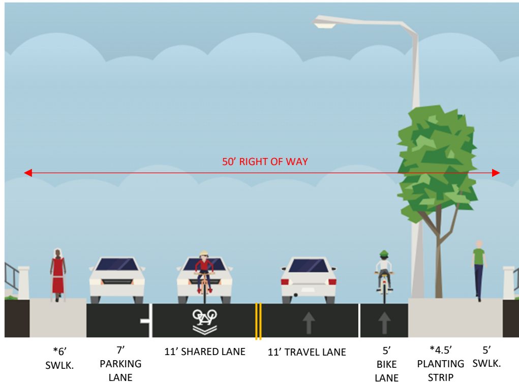
Proposed Layout – Option 2 – Uphill Bicycle Lanes
